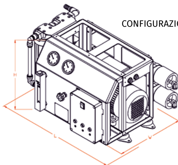
BOOSTER PUMP
