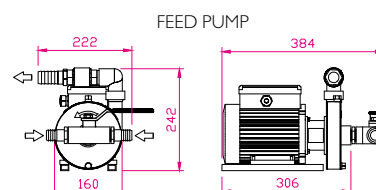
FEED PUMP
